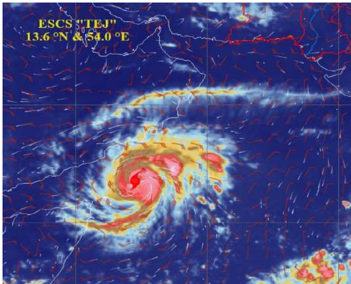
Satellite Imagery, 22 nd October 2023, 2000PST
