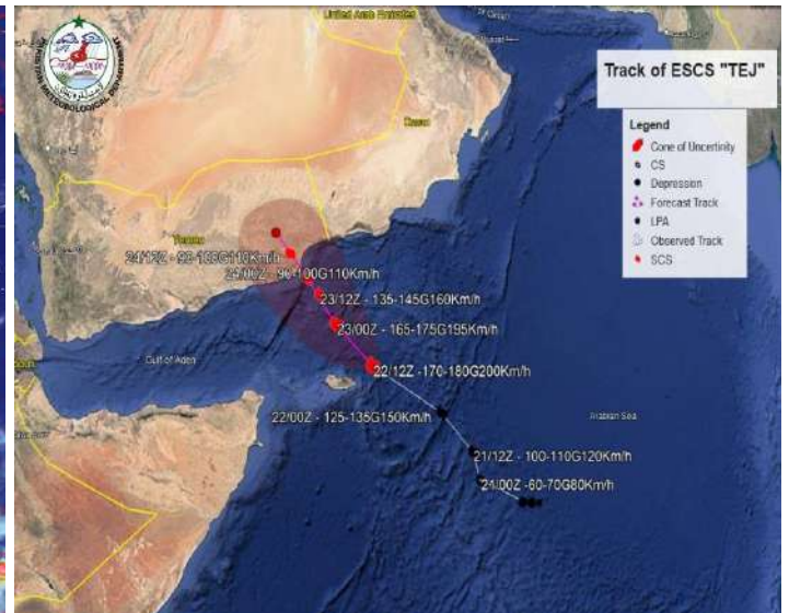
Observed and Forecast Track of Cyclone Sd/= Spokesman
